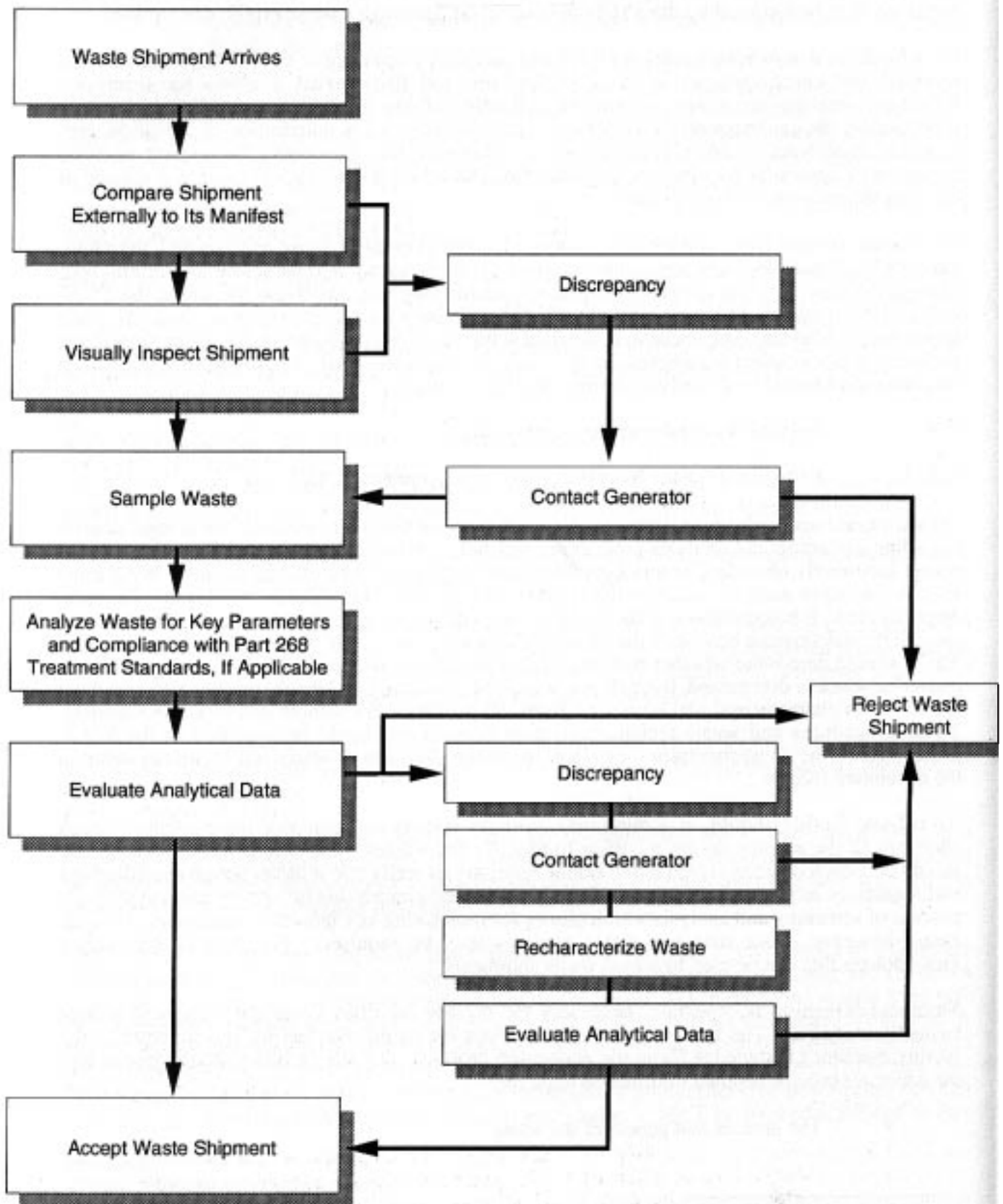
FIGURE 2-11 Shipment Screening
